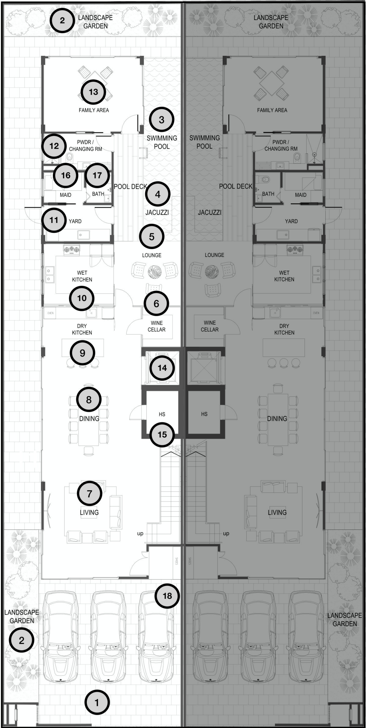
1ST STOREY PLAN
